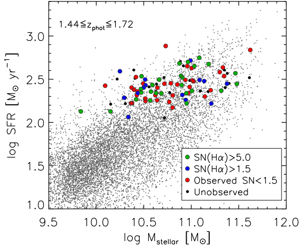
Figure 5. Herschel/PACS targets shown as a function of SFR and stellar mass. SFRs for PACS sources are based on 160\mu\text{m} fluxes. Galaxies observed with FMOS are marked in color indicative of whether a spectroscopic redshift was attained (same labels as in Figure 2). Herschel/PACS sources that not observed are marked as black circles. For comparison, we include the larger star-forming galaxy sample (small grey dots) with SFRs derived from SED fitting as described in the text.
