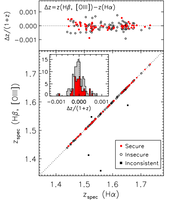
Figure 18. FMOS J-long confirmation of H\alpha -based spectroscopic redshifts. Symbols indicate whether at least one line is detected with a S/N \geq 3 (secure) or not (insecure). Filled squares indicate the insecure redshifts that are in disagreement.
