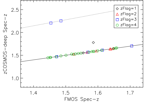
Figure 20. Comparison of spectroscopic redshifts between FMOS-COSMOS and zCOSMOS Deep surveys. FMOS redshifts are assessed separately by their quality flag as indicated. Only zCOSMOS deep redshifts having a secure (flag \geq 3 ) redshift are used for this comparison. The solid line represents a unity relation while the dashed line identifies where measurements will lie if [OIII]\lambda 5008 was mistaken for H\alpha .
