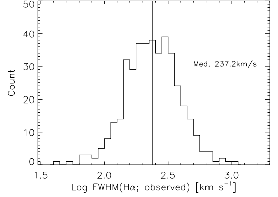
Figure 23. Distribution of the observed log FWHM of the H\alpha line (units of \text{km s}^{-1} ).
