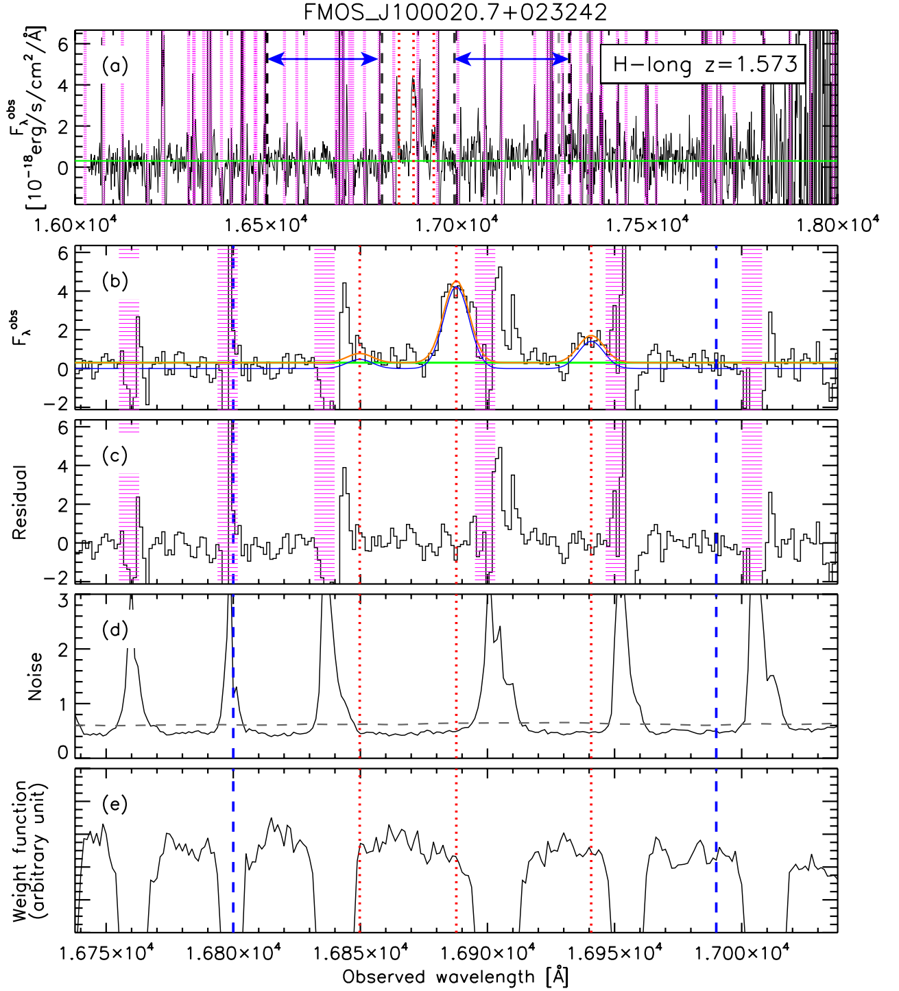
Figure 11. Example spectrum of a galaxy at z = 1.573 with a significant detection of H\alpha and [\text{NII}]\lambda 6585 as indicated by the vertical dotted lines (red). Individual panels are as follows: (a) Entire observed spectrum with regions impacted by OH lines shown in magenta. Two blue arrows indicate the regions used to determine the continuum level by fitting a linear function shown in green. (b) Observed spectrum over a narrower spectral range and centered on H\alpha . The overall fit to the spectrum is indicated in yellow with the components marked in green (continuum) and blue (emission lines). (c) Residual after subtracting the best-fit function to the emission lines and continuum. (d) RMS noise level and threshold (horizontal dashed line) for avoiding the wavelength range impacted by OH lines. (e) Weight function applied to each pixel for fitting both the continuum and emission lines.
