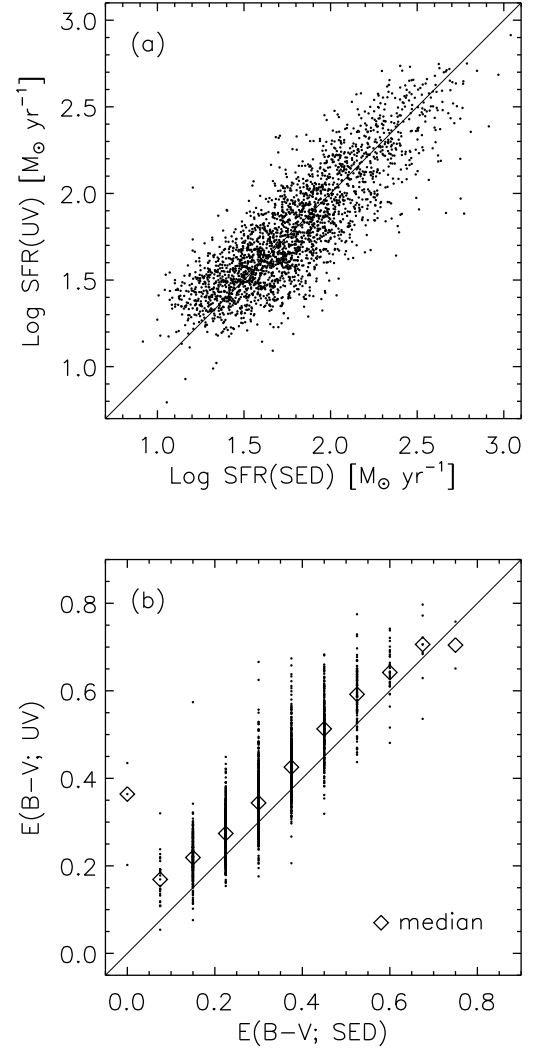
Figure 3. (a) Comparison of UV- and SED-based SFRs for the ‘very good’ sBzK sample. (b) Color excess as derived from B_J - z (UV) color and broad-band SED fitting.
