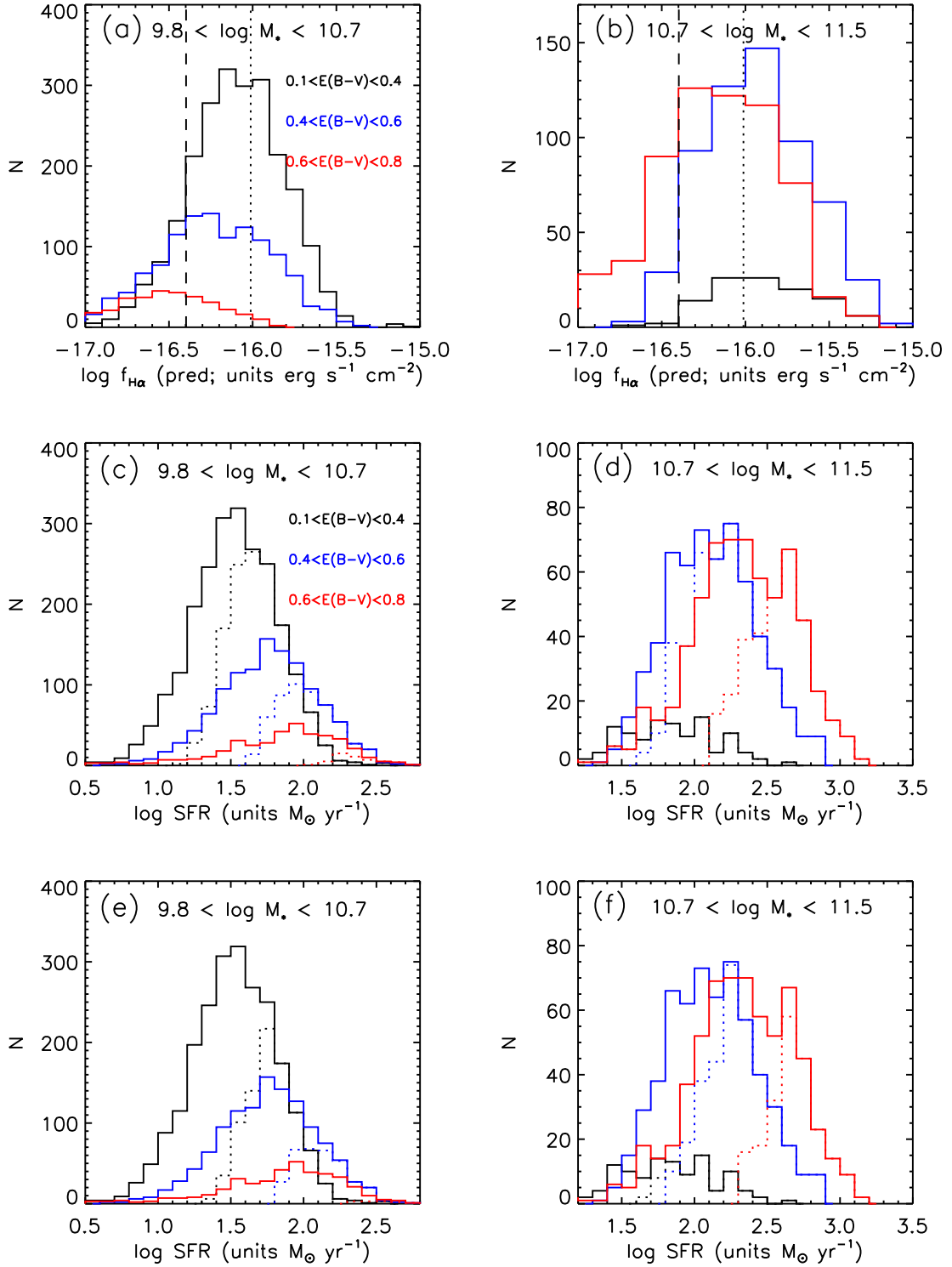
Figure 6. Target selection and impact of a weight on the predicted emission-line flux based on the parent photometric galaxy sample between 1.46 < z < 1.67 : (a) and (b) Distribution of predicted H \alpha emission-line flux (total; i.e., no consideration of the aperture size) split in bins of stellar mass and color excess as indicated. The vertical dashed lines show our imposed limits on line flux (see text for details). (c – f) SFR distribution in bins of stellar mass and color excess. The solid histograms are the full sample while the dashed histograms represent the sample with the imposition of a limit on H \alpha emission-line flux (panels c – d: f_{\text{H}\alpha} > 4 \times 10^{-17} \text{ erg cm}^{-2} \text{ s}^{-1} ; panels e – f: f_{\text{H}\alpha} > 1 \times 10^{-16} \text{ erg cm}^{-2} \text{ s}^{-1} ) for each bin of color excess.
