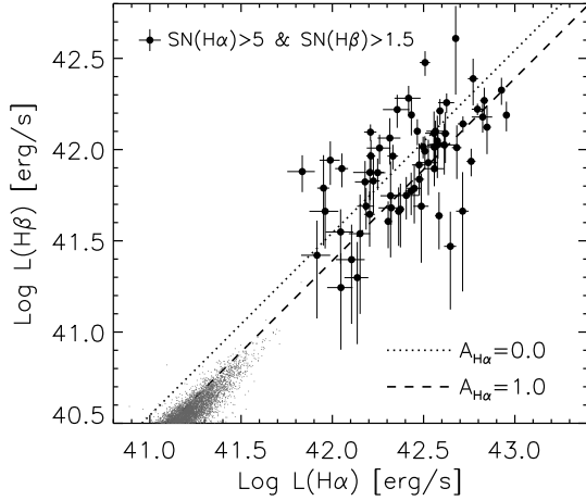
Figure 26. Emission-line luminosities ( H\alpha versus H\beta ) of our secure sample ( H\alpha S/N > 5 ; H\beta S/N > 1.5 ; OH impact < 50\% ). For reference, we plot values from SDSS as small grey dots. We indicate the expected values with ( A_{H\alpha} = 1 ) and without extinction.
