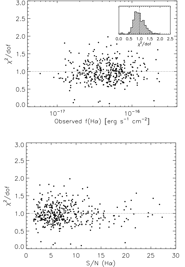
Figure 13. Assessing the accuracy of our line-fitting routine. The reduced chi-square statistic of each fitted H\alpha line as a function of observed H\alpha flux (top panel) and S/N (bottom panel).
