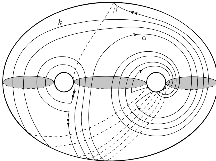
Figure 1: The curve k is a band sum of \alpha and \beta , and is complicated with respect to the indicated maximal meridian system in the sense of Kobayashi.
