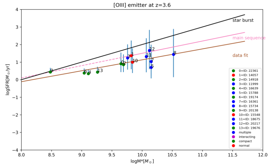
SFR-M* relation
