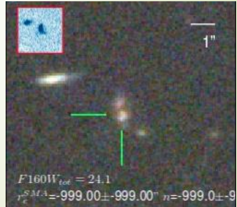
15734(from HST)
