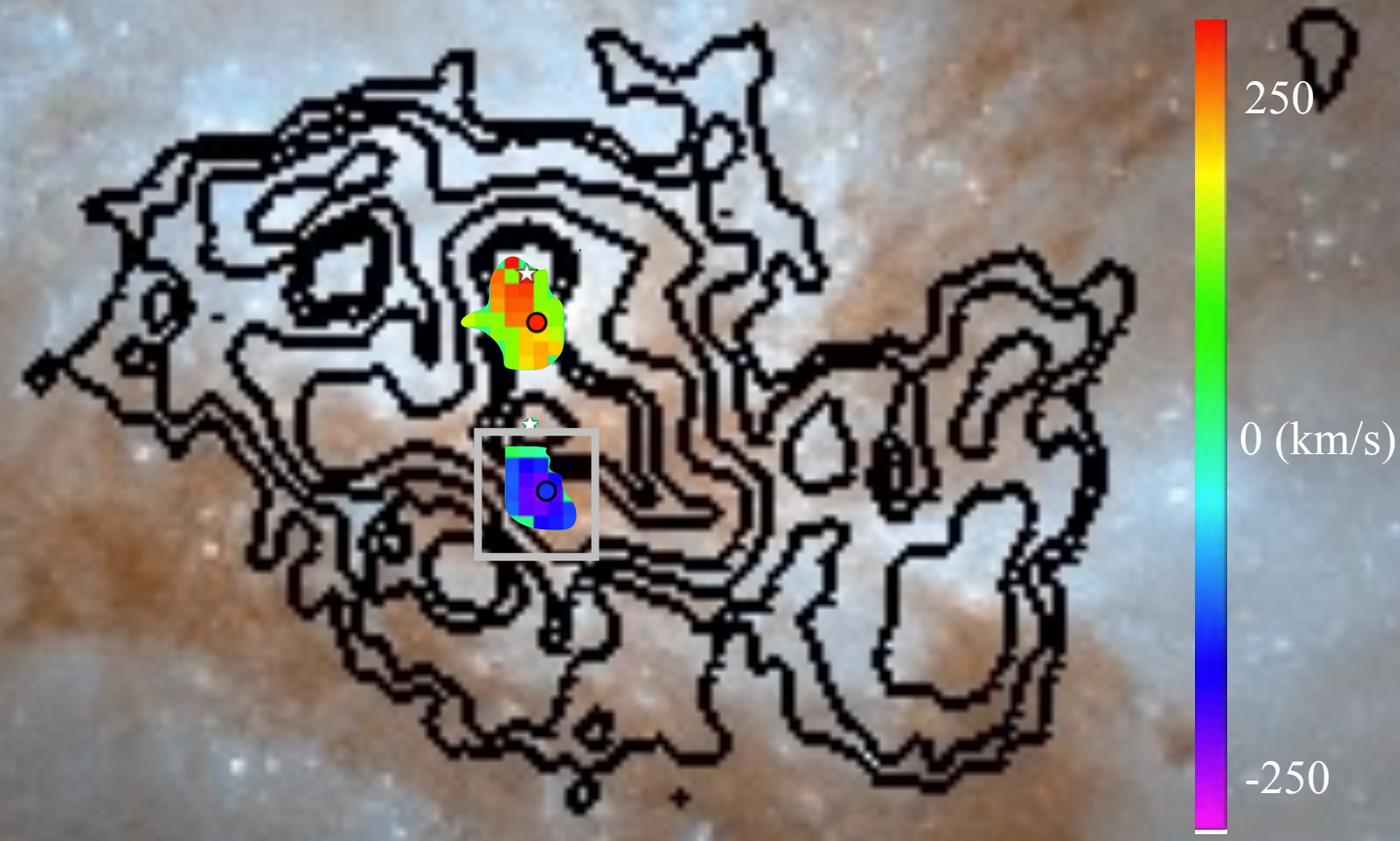
Velocity map for HCN(1-0) broad components (contour: 13 CO(1-0), background HST 3-color map)
