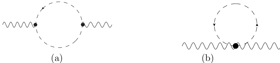
Figure 1: Scalar loop contributions to the photon vacuum polarization.
