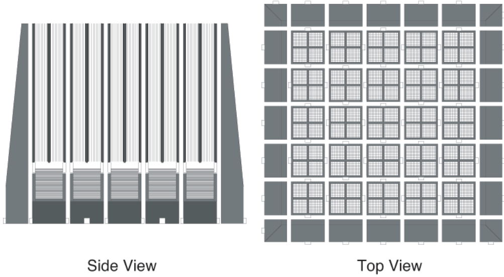
Fig. 9. A schematic drawing of the SGD. It consists of 25 units of the narrow FOV Compton telescope surrounded by 24 shield counters made of BGO. A geometrical area of 525 \text{ cm}^2 is currently assumed for the sum of 25 units. If we select an event that has two hits in the detector (and no hit in the BGO shields) and if we require the proper reconstruction for the Compton kinematics, the effective area at 200 keV becomes \sim 100 \text{ cm}^2 , including the reconstruction efficiency.
