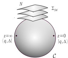
Figure 1: \Sigma_{SW} as an N -fold cover of \mathcal{C}
